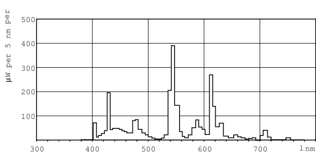
LDPB_TL5-HO8_850-Spectral power distribution B/W
