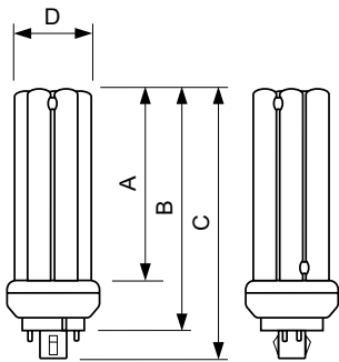
PL-T 32W/841/A/4P/ALTO
